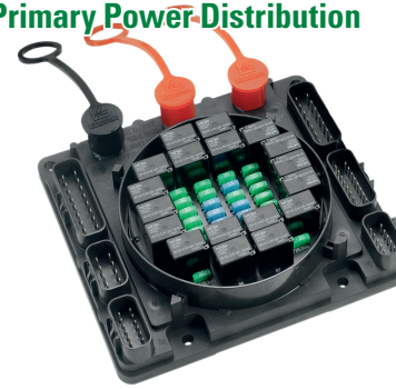
FLEC3000Z-0 - FLEC Series
